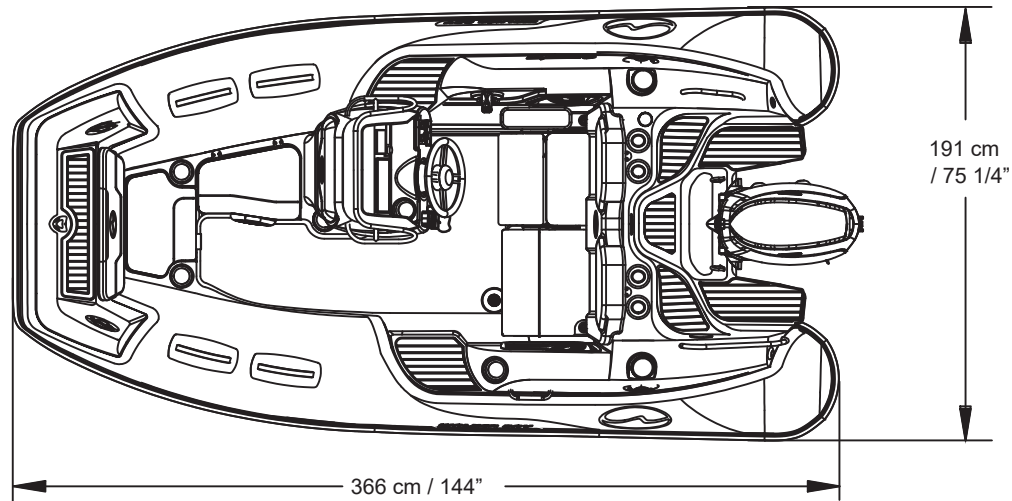
Top View
